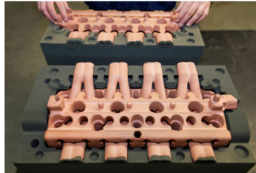
3D printed sand moulds and cores assembly
