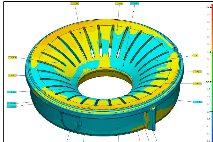
3D scan and comparison between 3D design and raw casting
