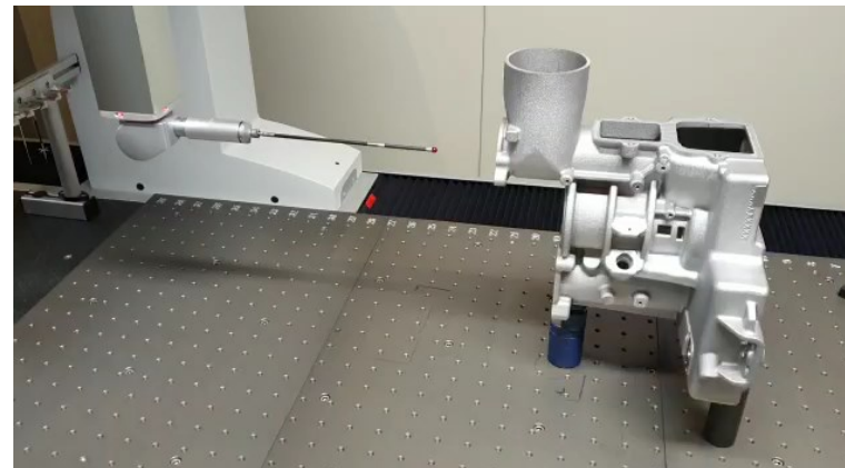
Dimensional control of the machined area
